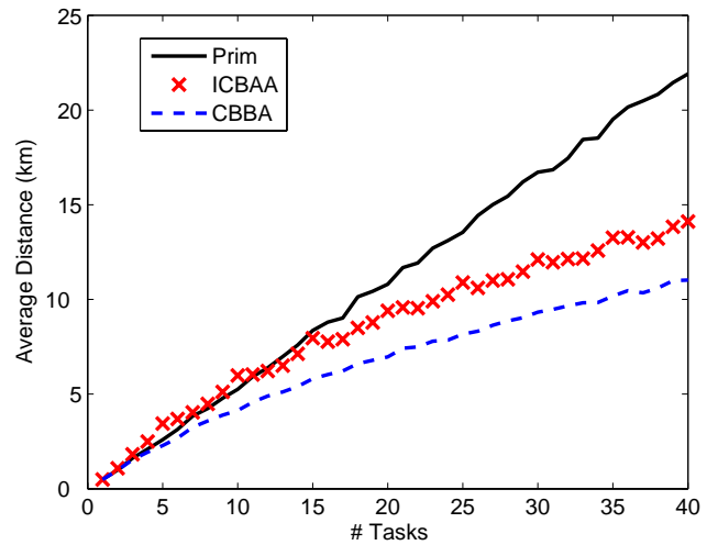
Fig. 3. The total distance traveled to accomplish assignment ( N_u = 5 )
