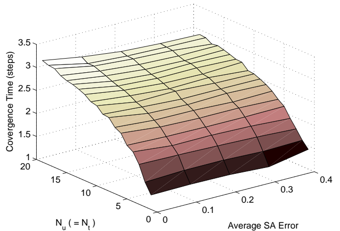
Fig. 1. Convergence of CBBA in the presence of inconsistency in situational awareness
