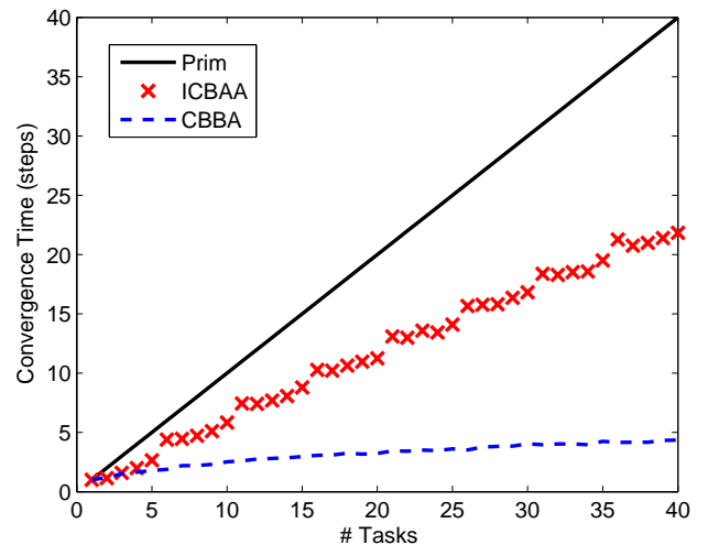
Fig. 4. Convergence time steps ( N_u = 5 )
