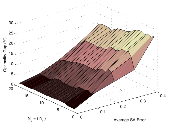
Fig. 2. Optimality gap of CBBA in the presence of inconsistency in situational awareness
