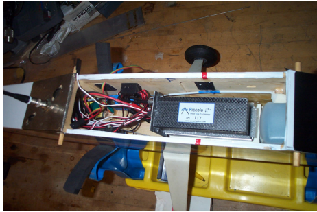
Fig. 11. Piccolo autopilot from Cloud Cap Tech.
