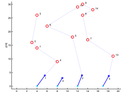
Fig. 6. Plan after first re-assignment (rover 4 is lost)
