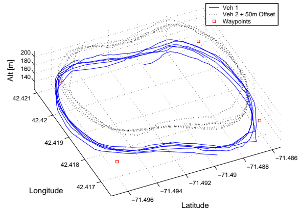
Fig. 13. Autonomous UAV flight data.
