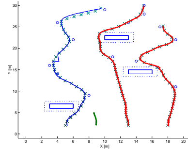
Fig. 8. Rover trajectories as measured during the experiment
