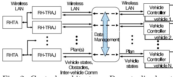
Fig. 2. Control architecture: Decentralized path planning/Distributed task assignment.
