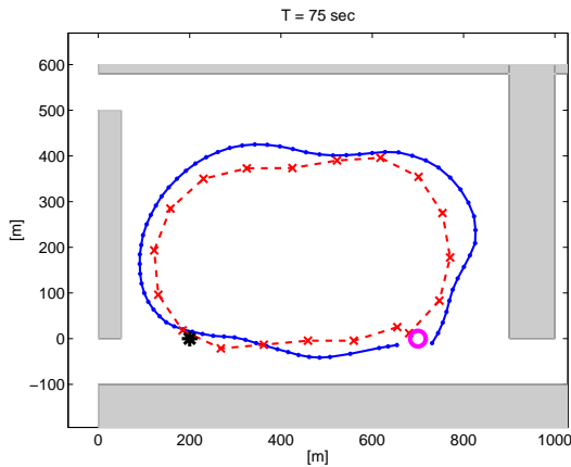
Fig. 16. Completion of the circuit- Wind disturbances are \sim 5 m/s (W to E).
