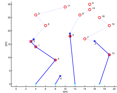
Fig. 7. Last assignment (new tasks at wpts 15 and 16 appear)
