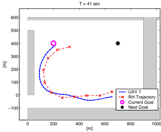
Fig. 14. Demonstration of UAV receding horizon control 41 seconds into the circuit. Planned paths are the dashed lines, vehicle telemetry shown by solid lines.
