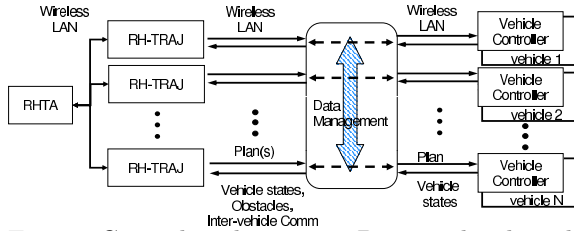
Fig. 3. Control architecture: Decentralized path planning/Centralized task assignment.
